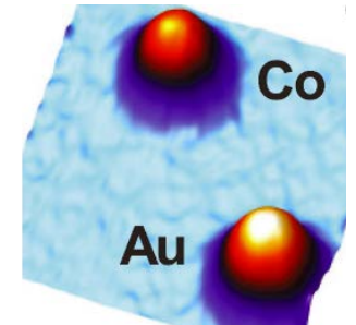
Adsorbed atoms
