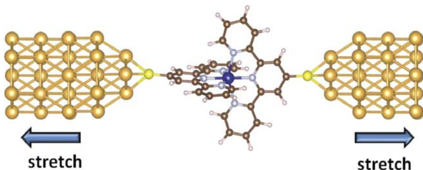
Au—Co(tpy-S) 2 —Au
