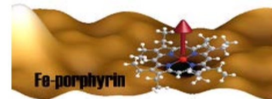
Molecular spintronics
