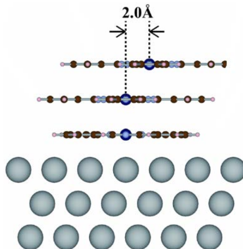
few-layer CoPc/Pb(111)
