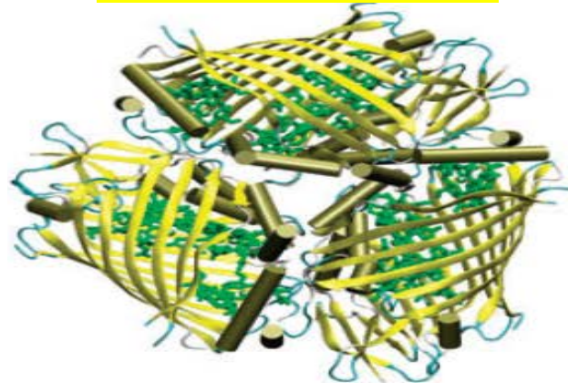
Molecular spintronics
