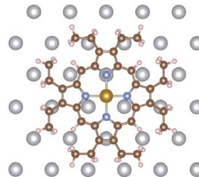
FeOEP/Pb(111)
